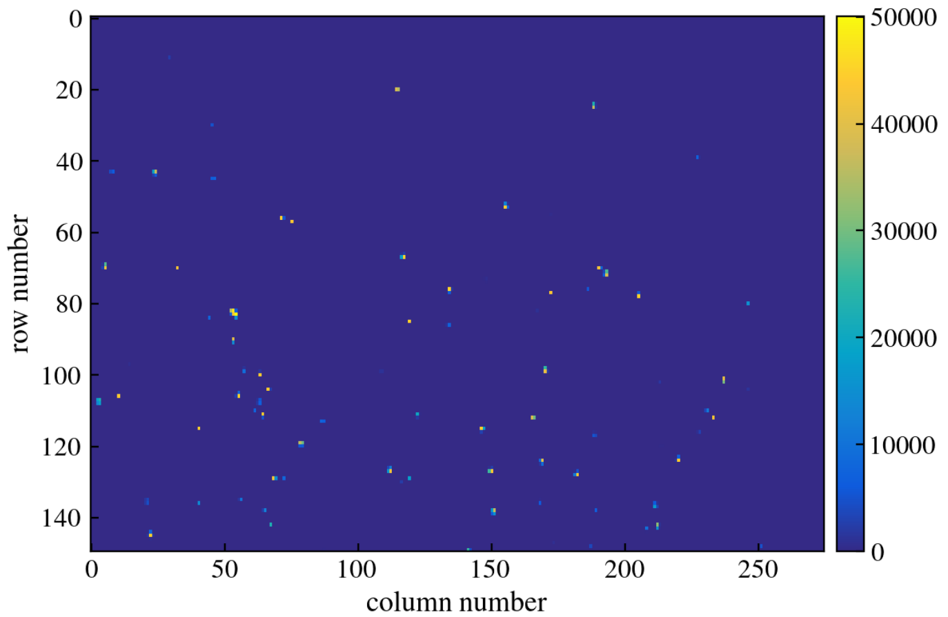
Figure 303: CCD Image
