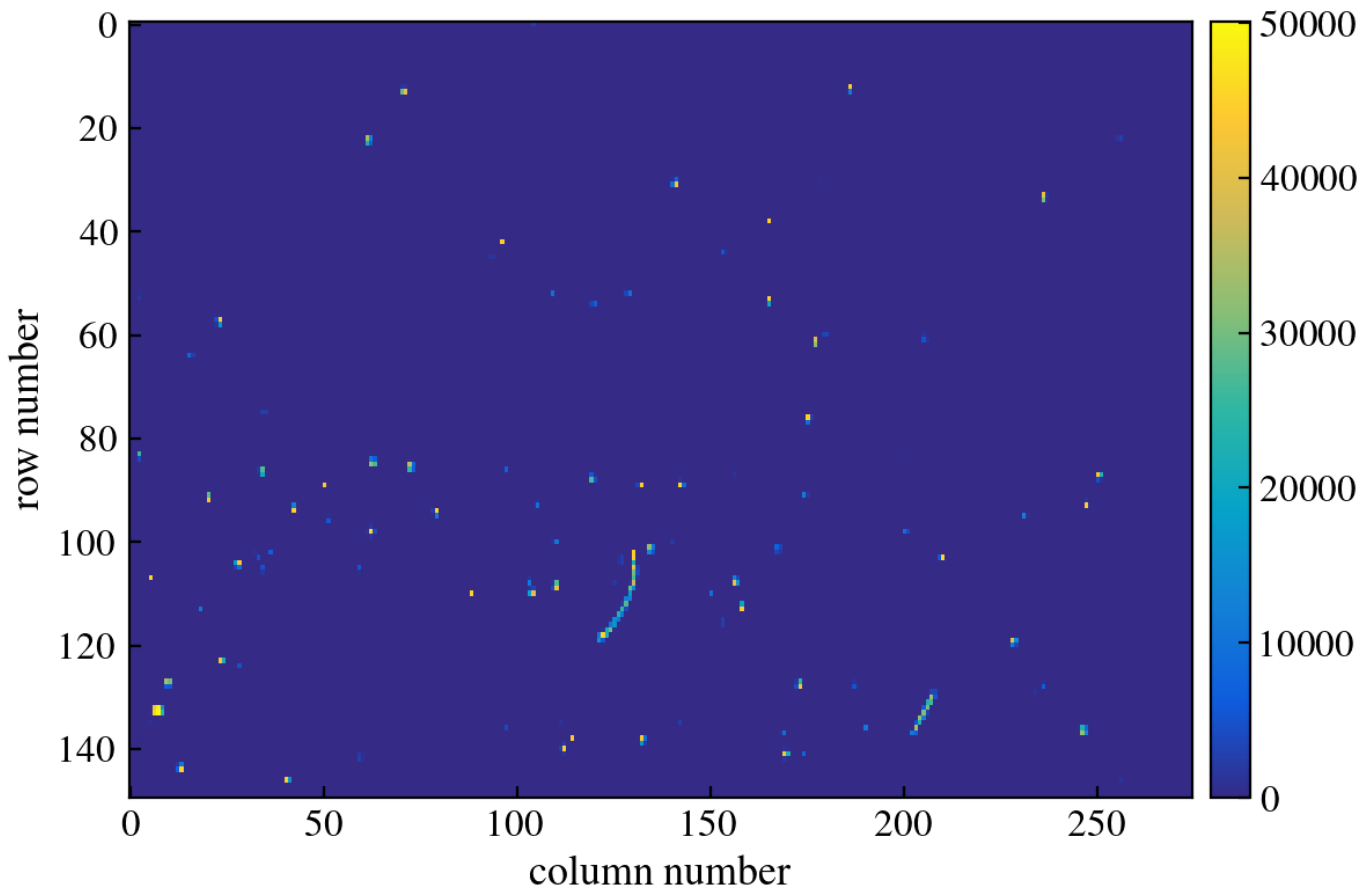
Figure 232: CCD Image
