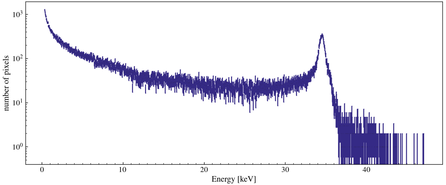
Single Pixel Energy Distribution [w/ 4.84 ADC/e- and 3.74eV/e-] [class MESinglePED]
