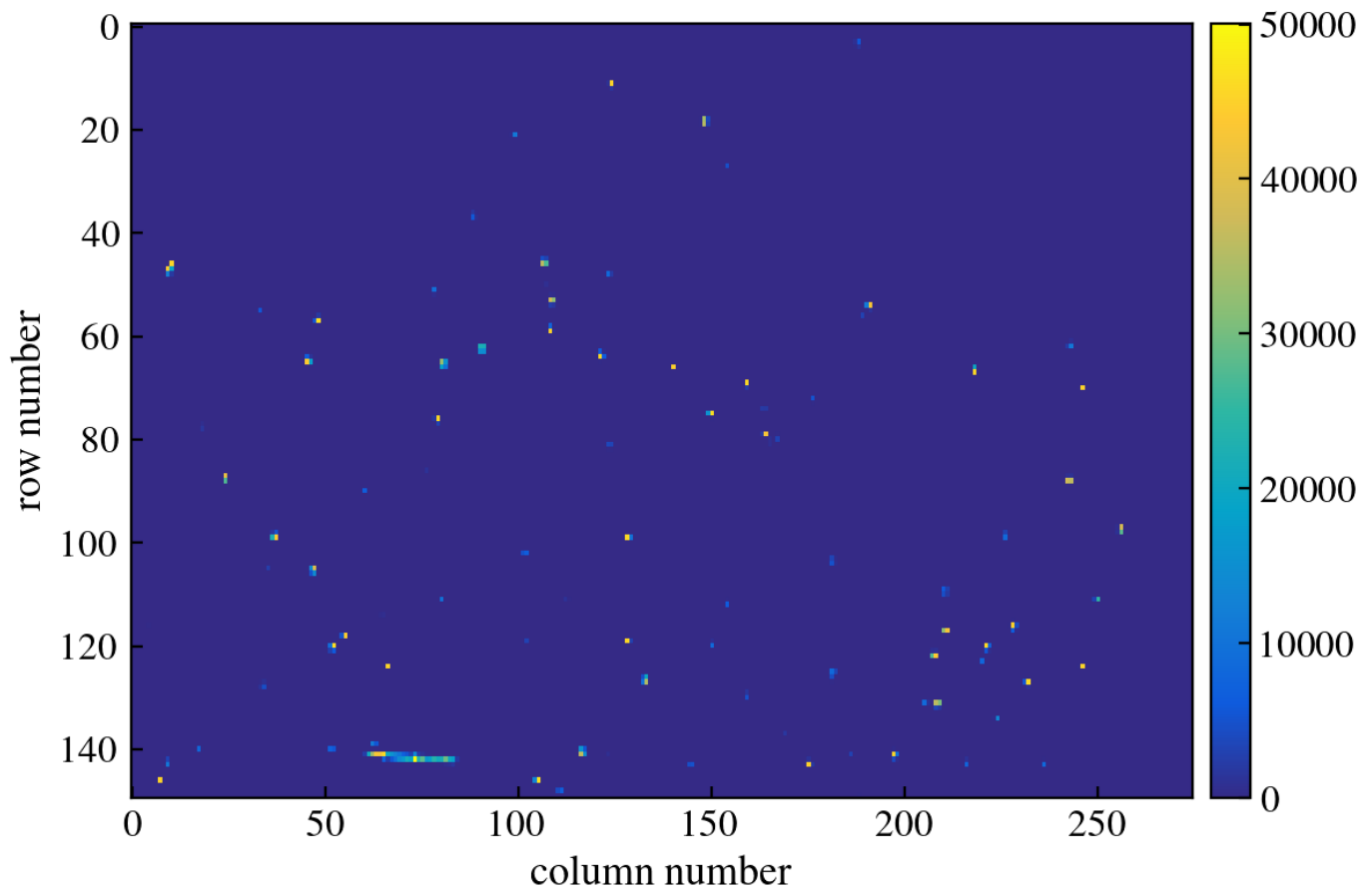
Figure 83: CCD Image
