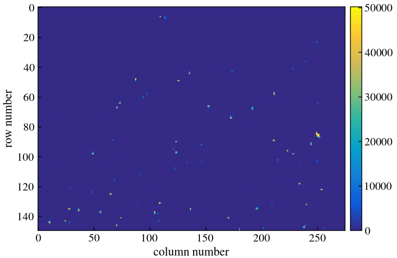
Figure 191: CCD Image
