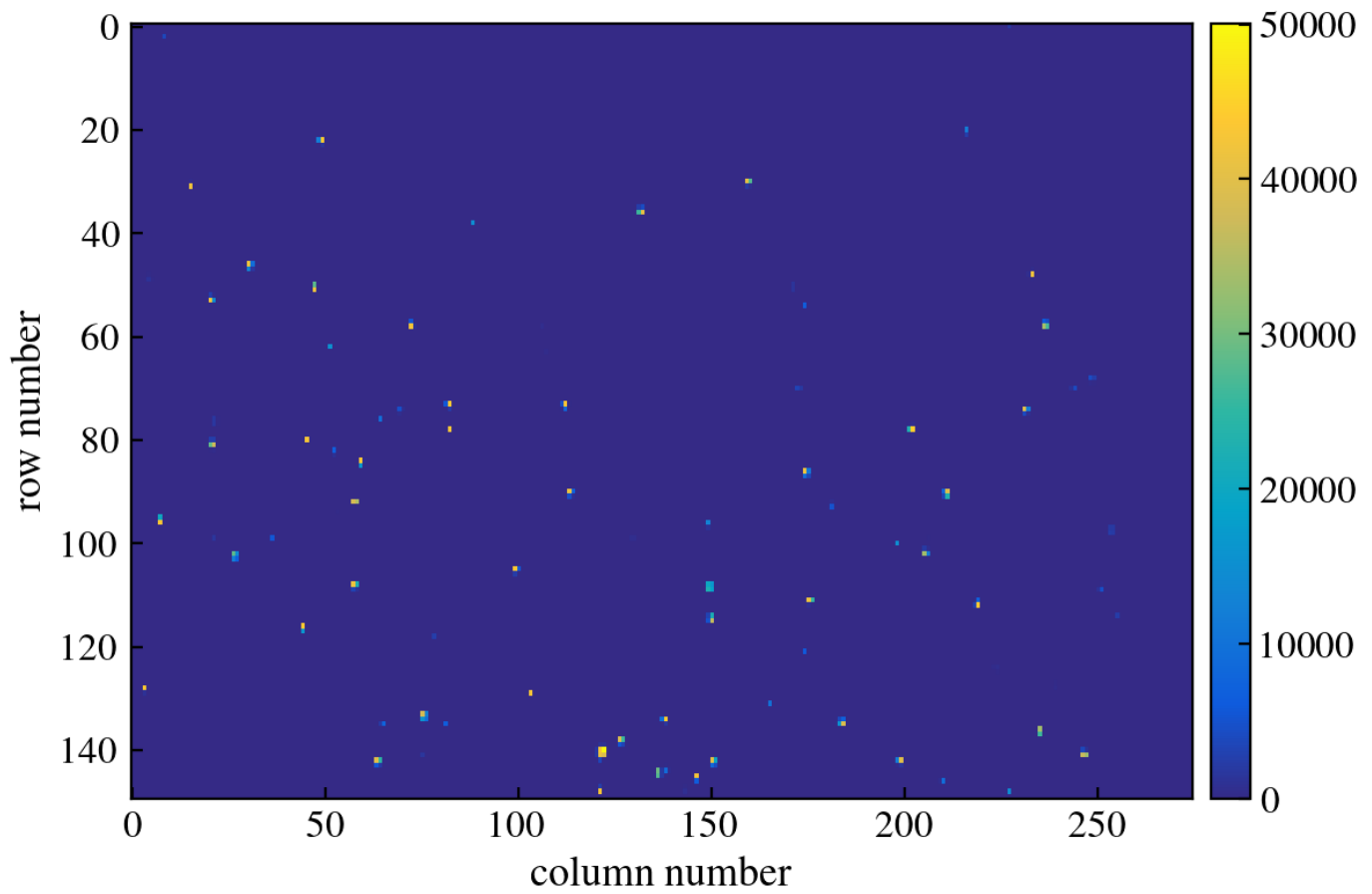
Figure 315: CCD Image
