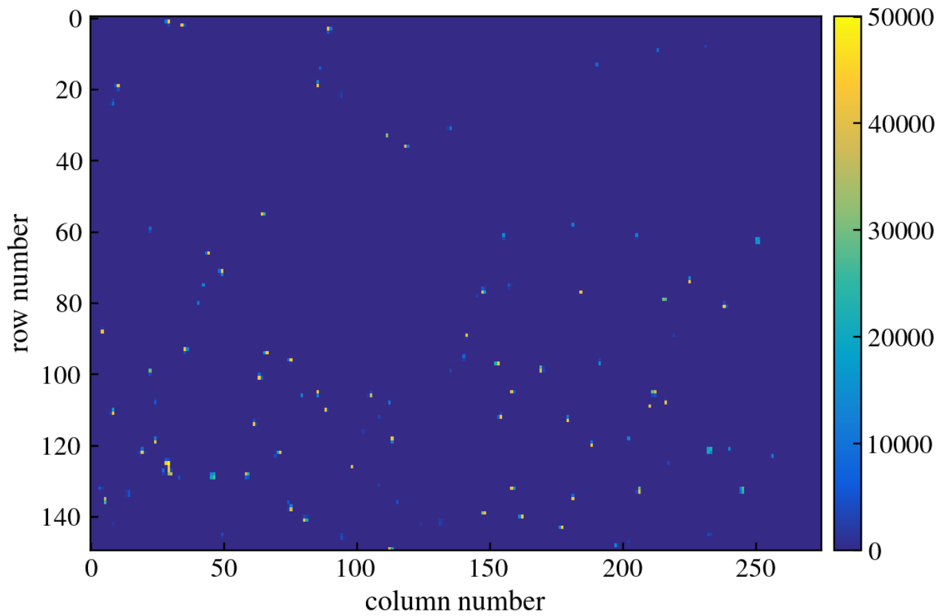
Figure 189: CCD Image
