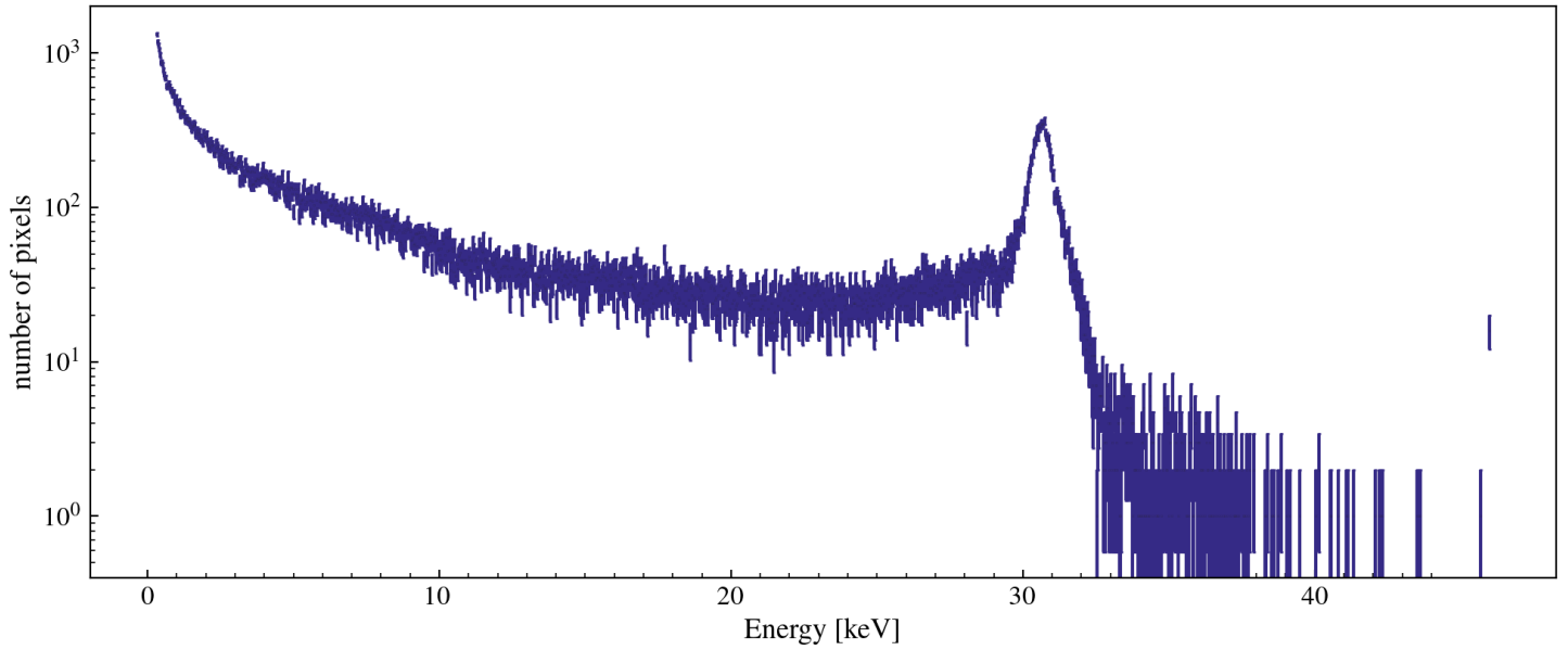
Single Pixel Energy Distribution [w/ 5.24 ADC/e- and 3.74eV/e-] [class MESinglePED]
