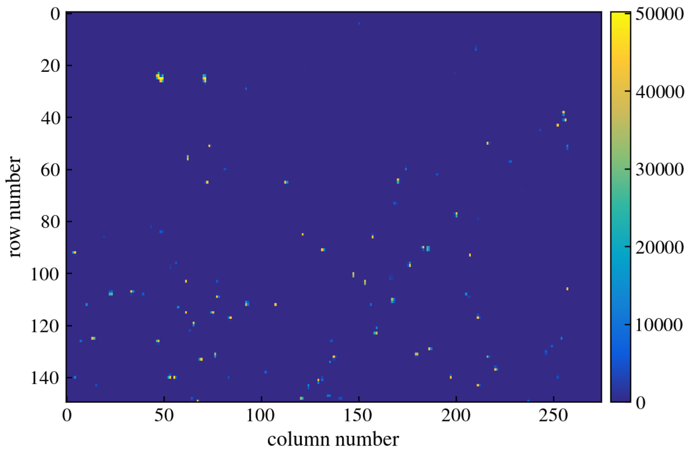
Figure 198: CCD Image
