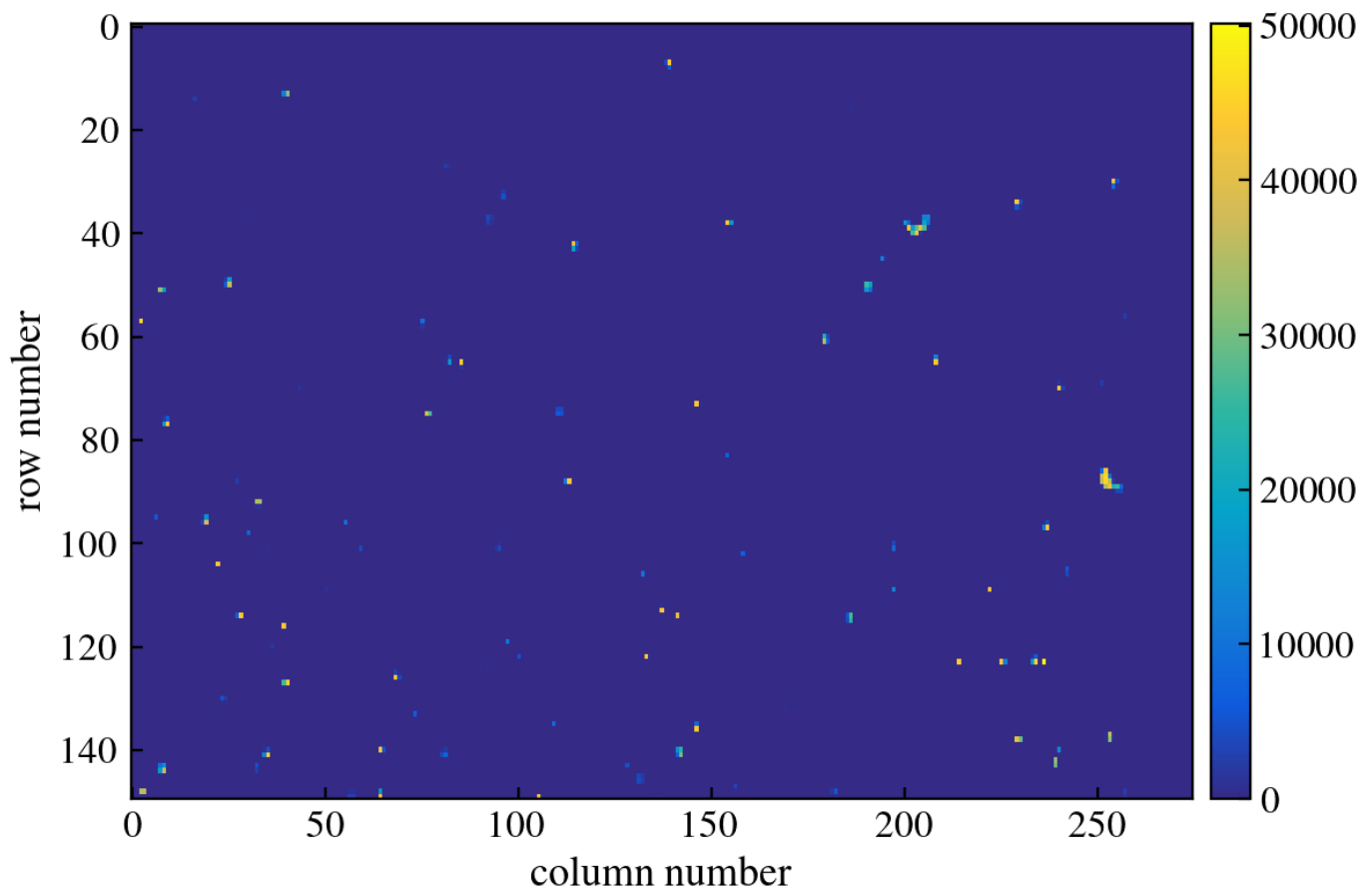
Figure 74: CCD Image
