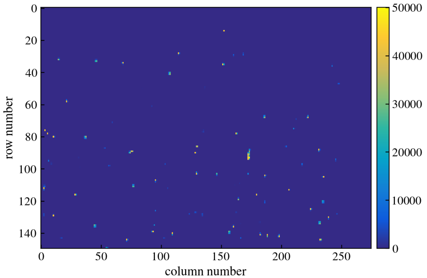
Figure 122: CCD Image
