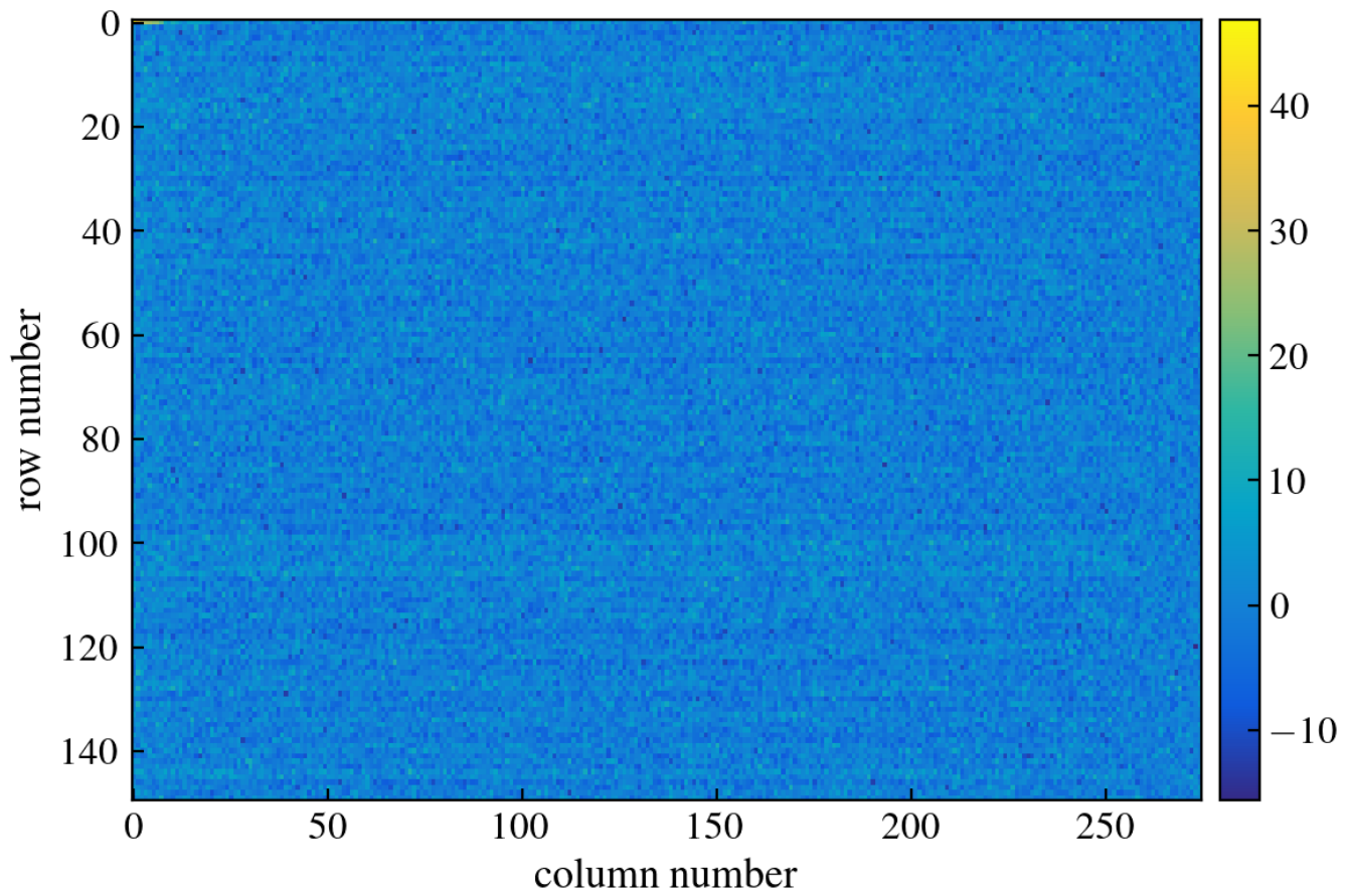
Figure 278: CCD Image
