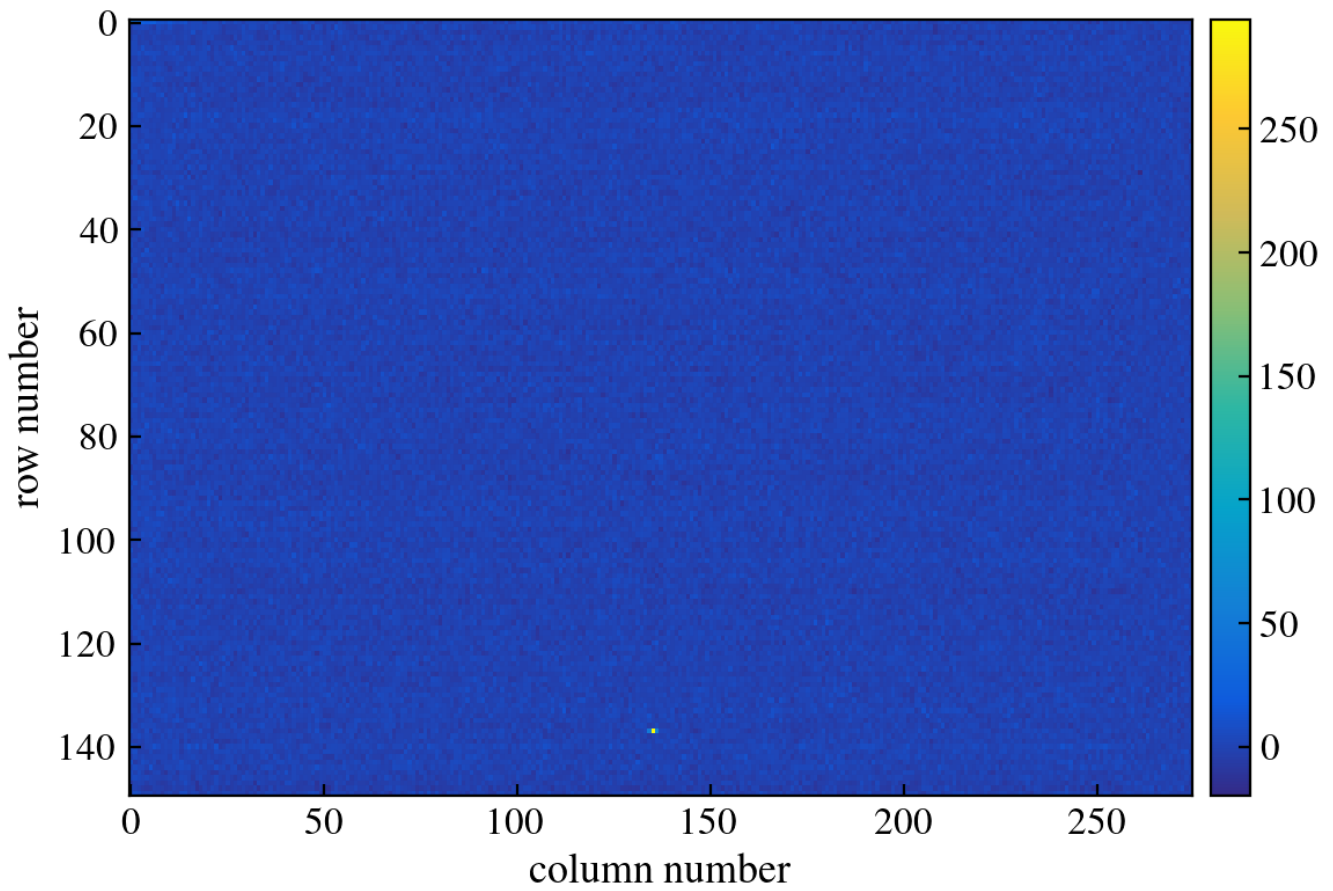
Figure 352: CCD Image
