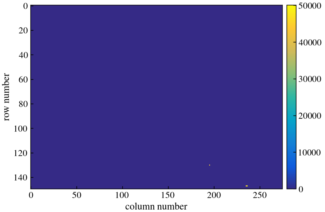
Figure 402: CCD Image
