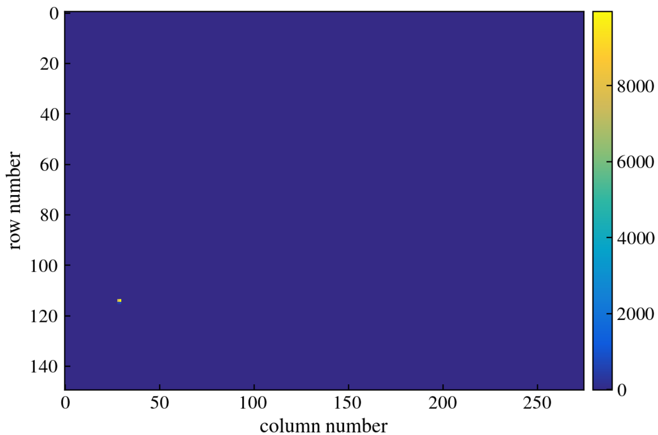
Figure 32: CCD Image
