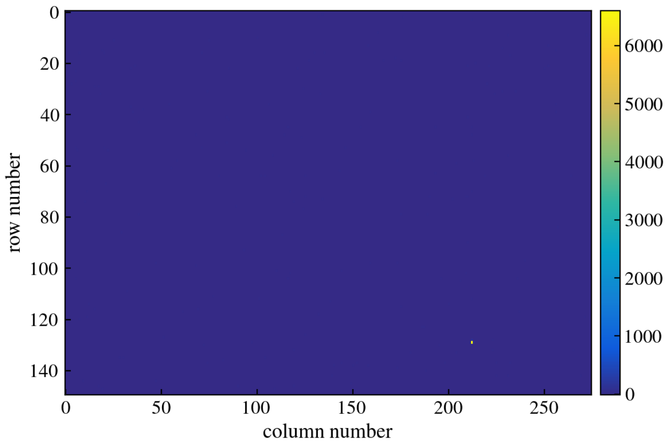
Figure 112: CCD Image
