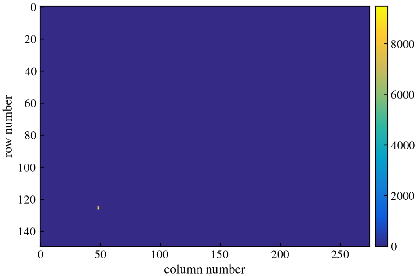
Figure 256: CCD Image
