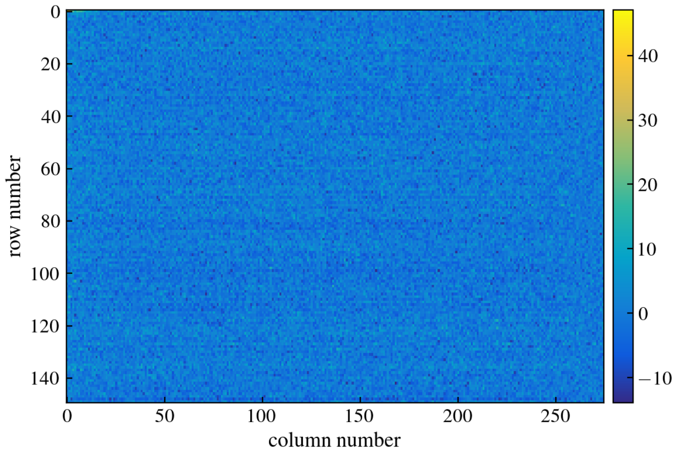
Figure 128: CCD Image
