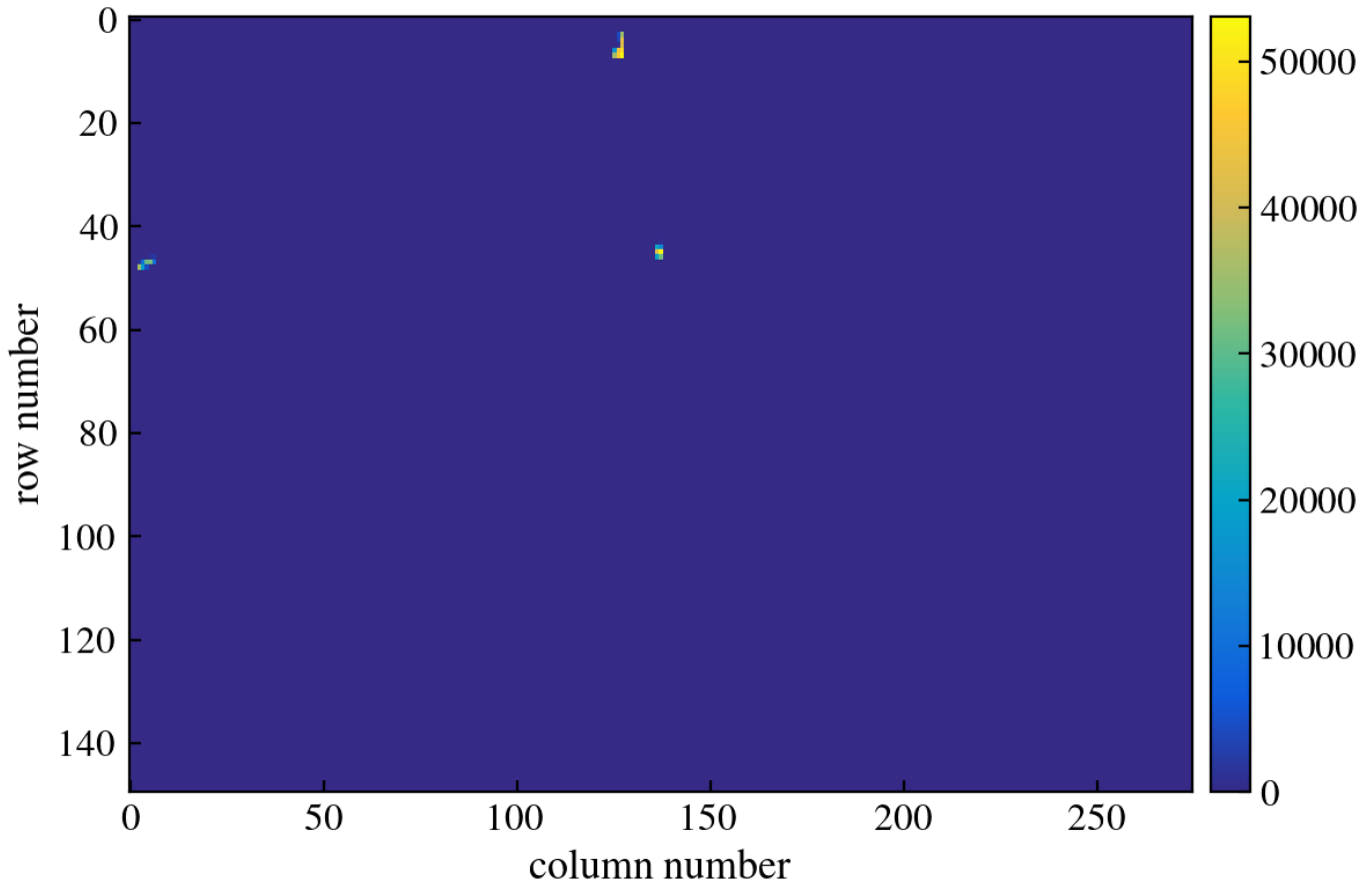
Figure 384: CCD Image
