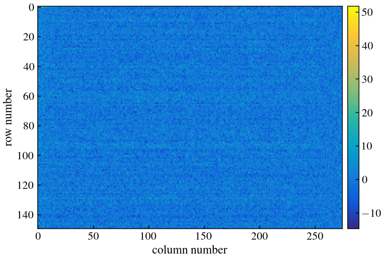
Figure 280: CCD Image
