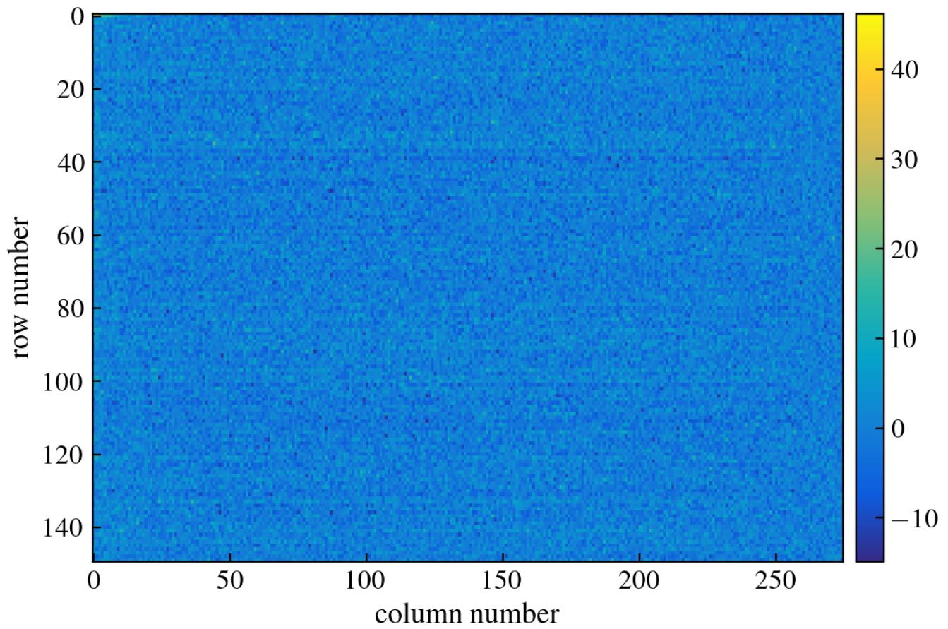
Figure 47: CCD Image
