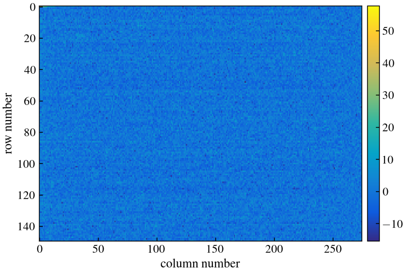
Figure 321: CCD Image
