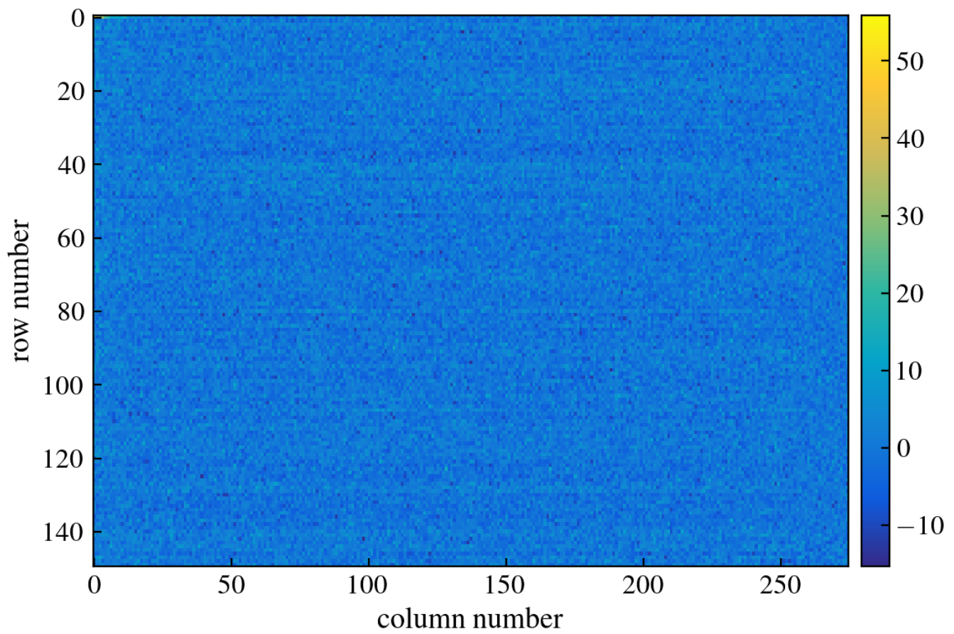
Figure 159: CCD Image
