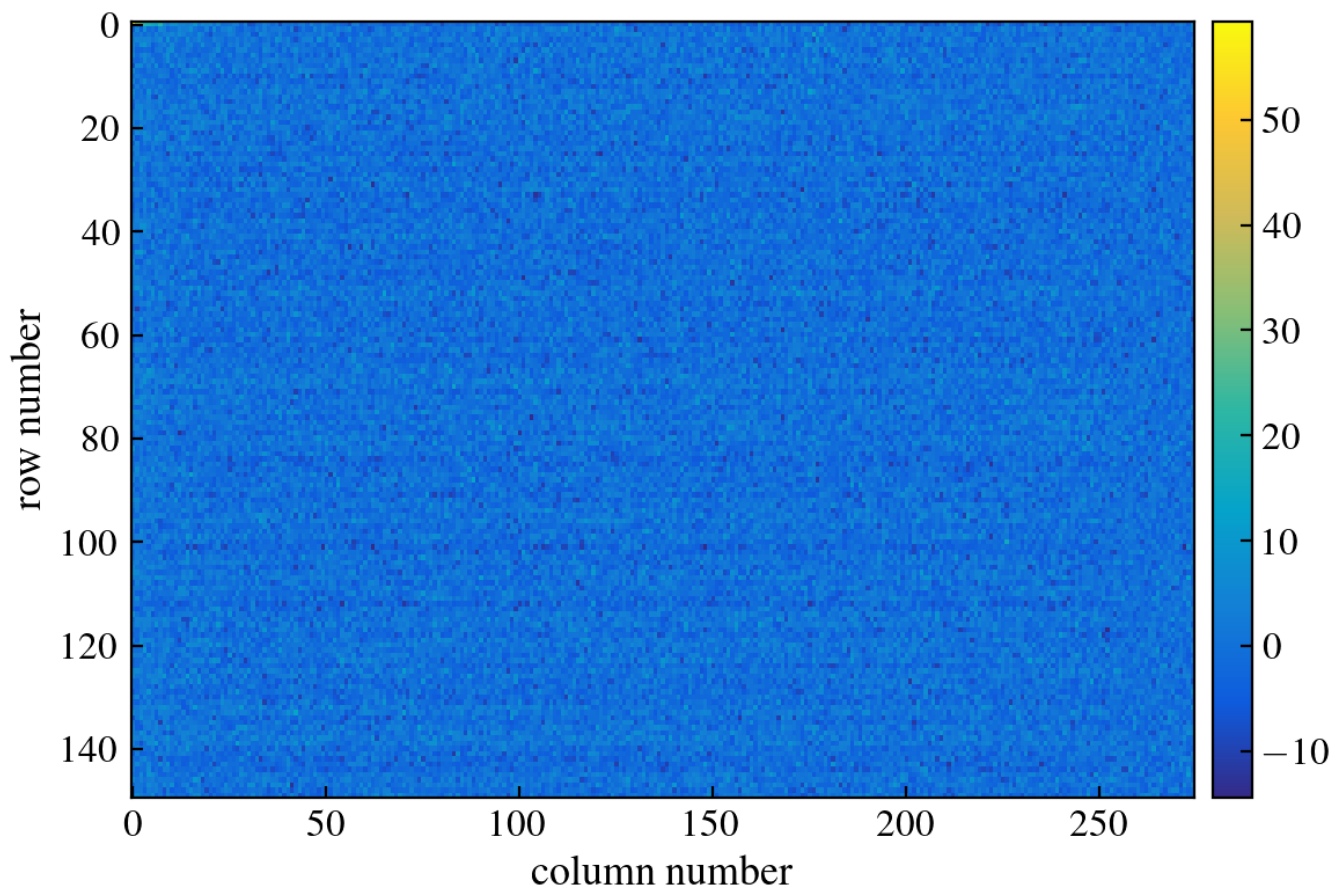
Figure 59: CCD Image
