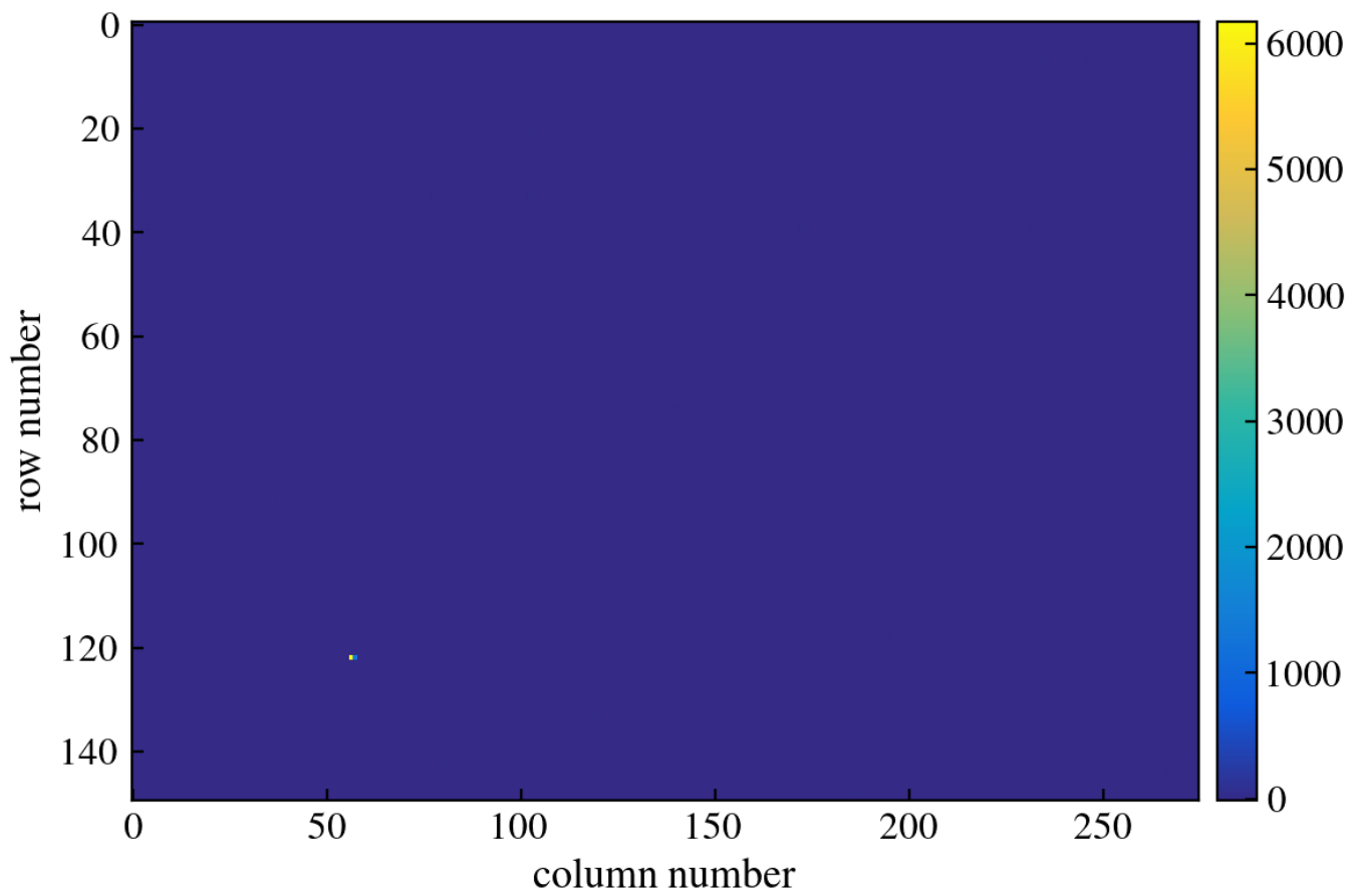
Figure 93: CCD Image
