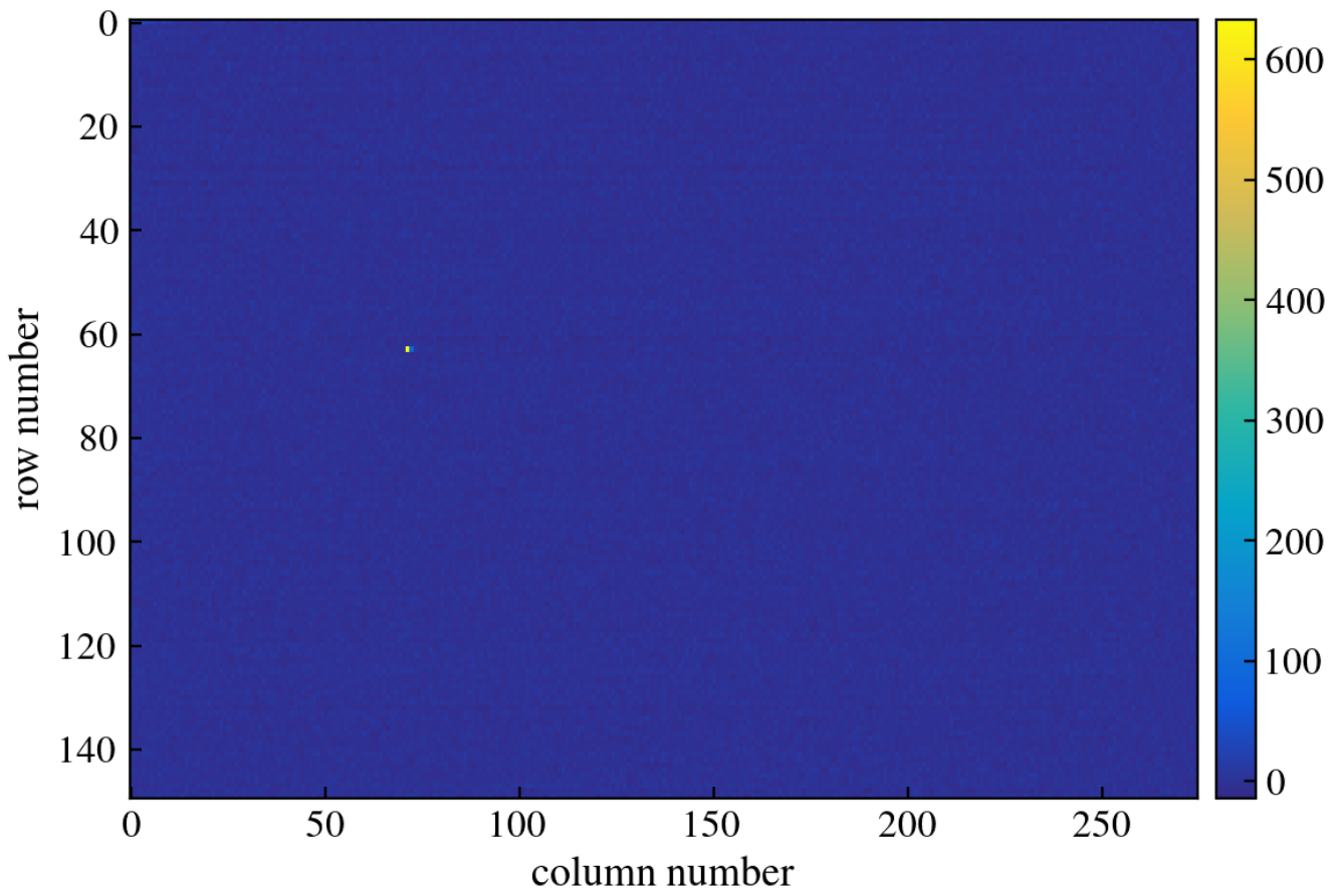
Figure 318: CCD Image
