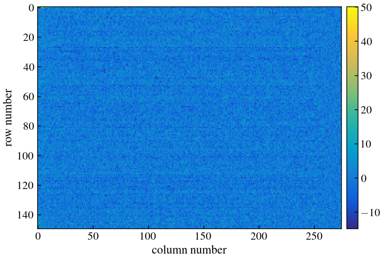
Figure 61: CCD Image
