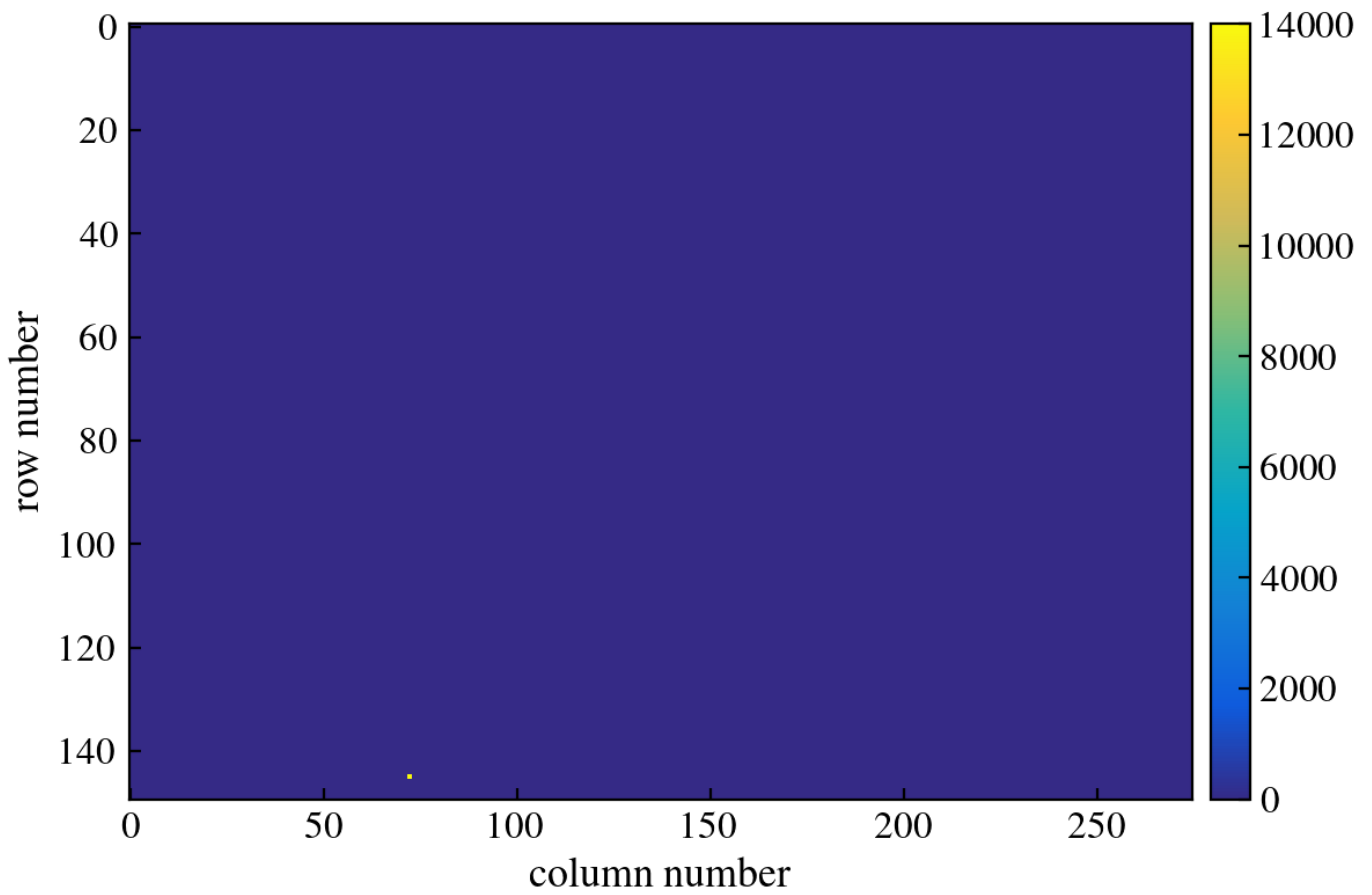
Figure 415: CCD Image
