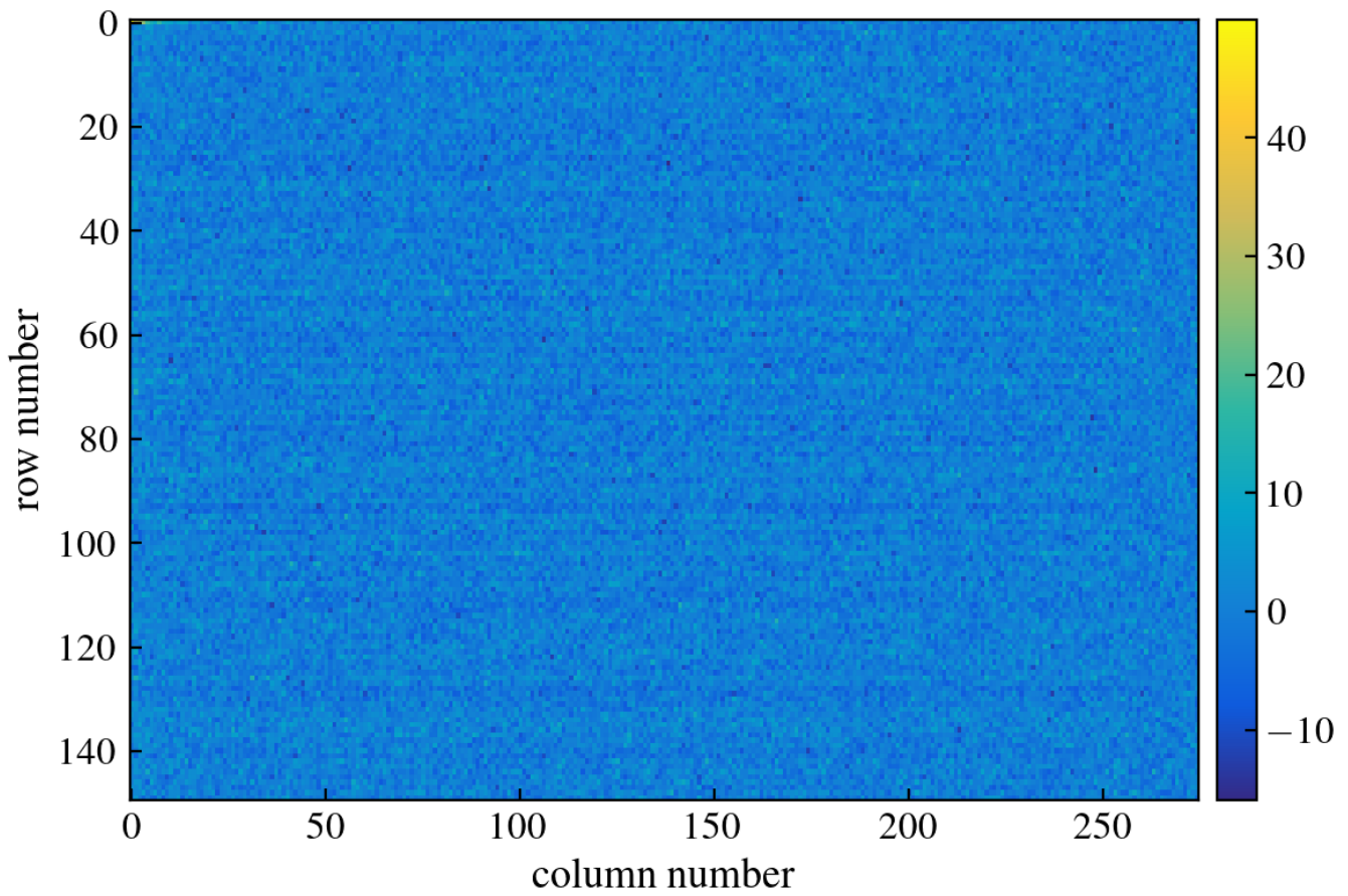
Figure 203: CCD Image
