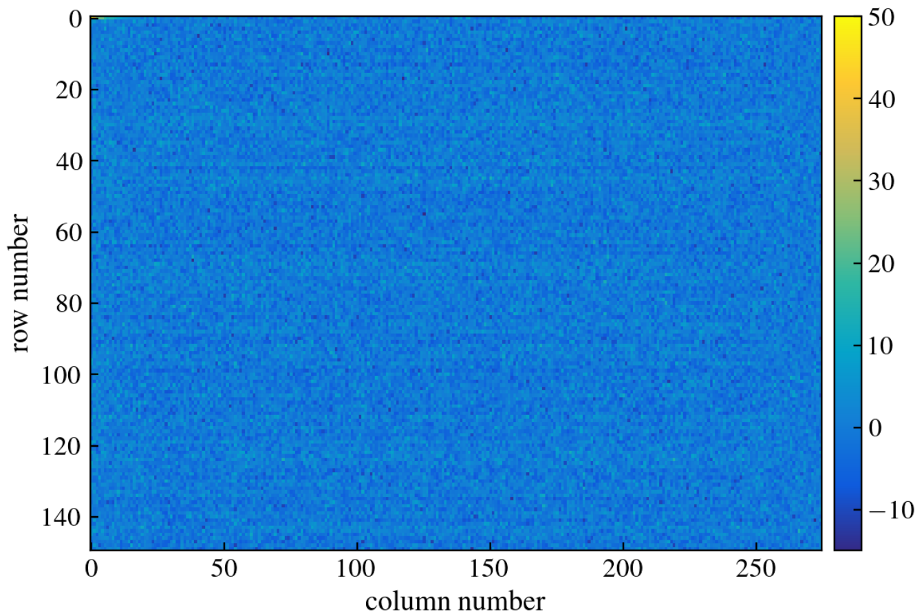
Figure 52: CCD Image
