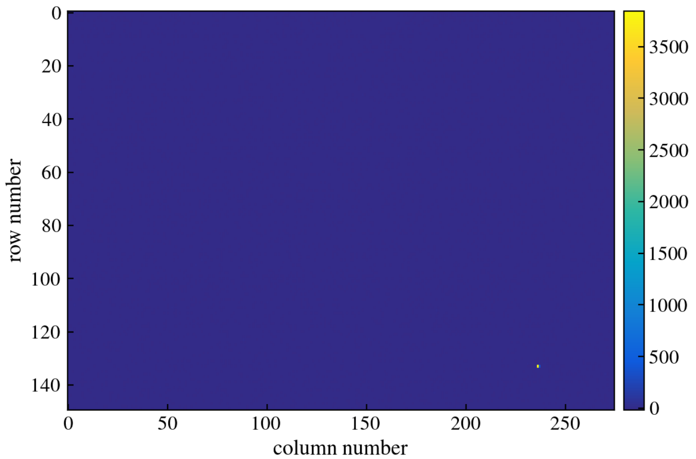
Figure 53: CCD Image
