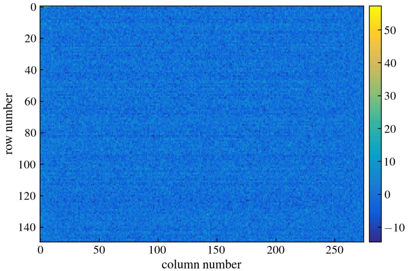
Figure 325: CCD Image
