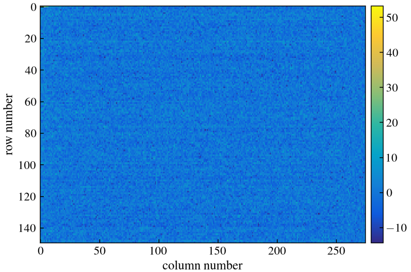
Figure 240: CCD Image
