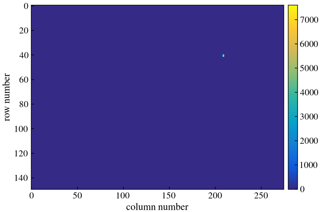
Figure 156: CCD Image
