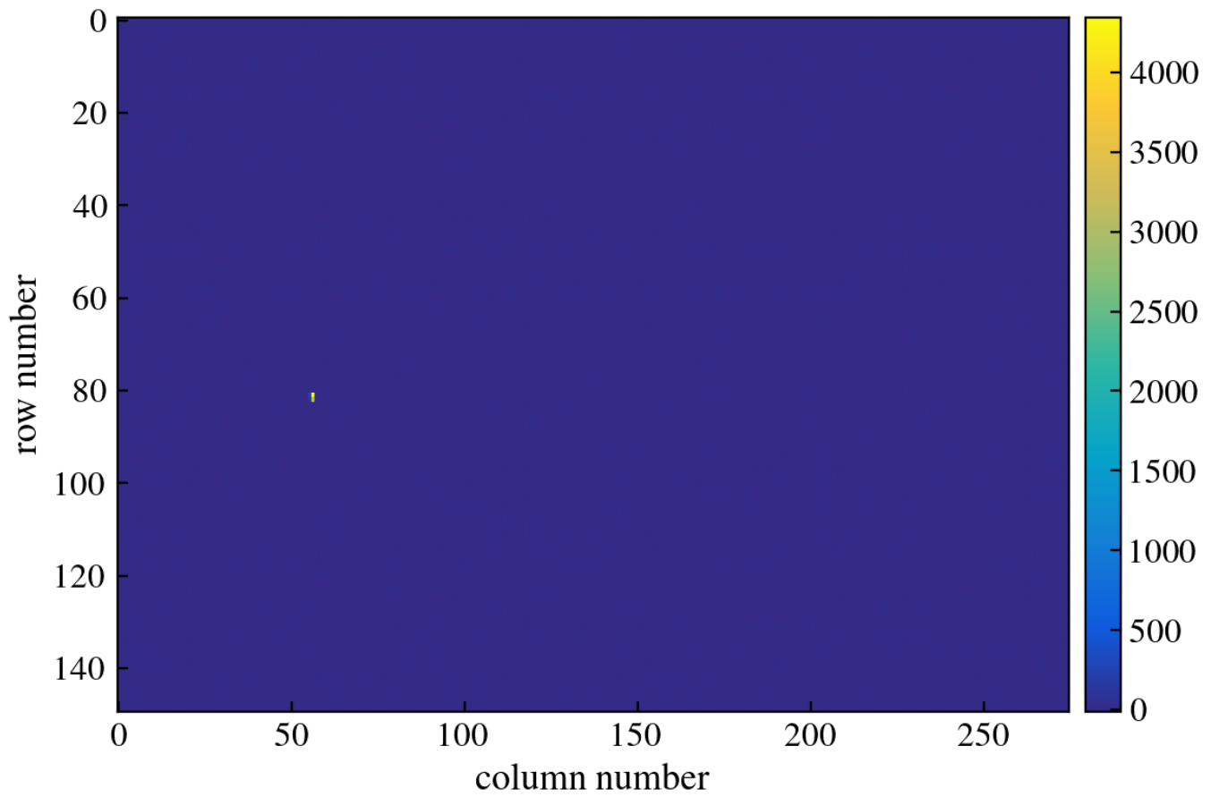
Figure 329: CCD Image
