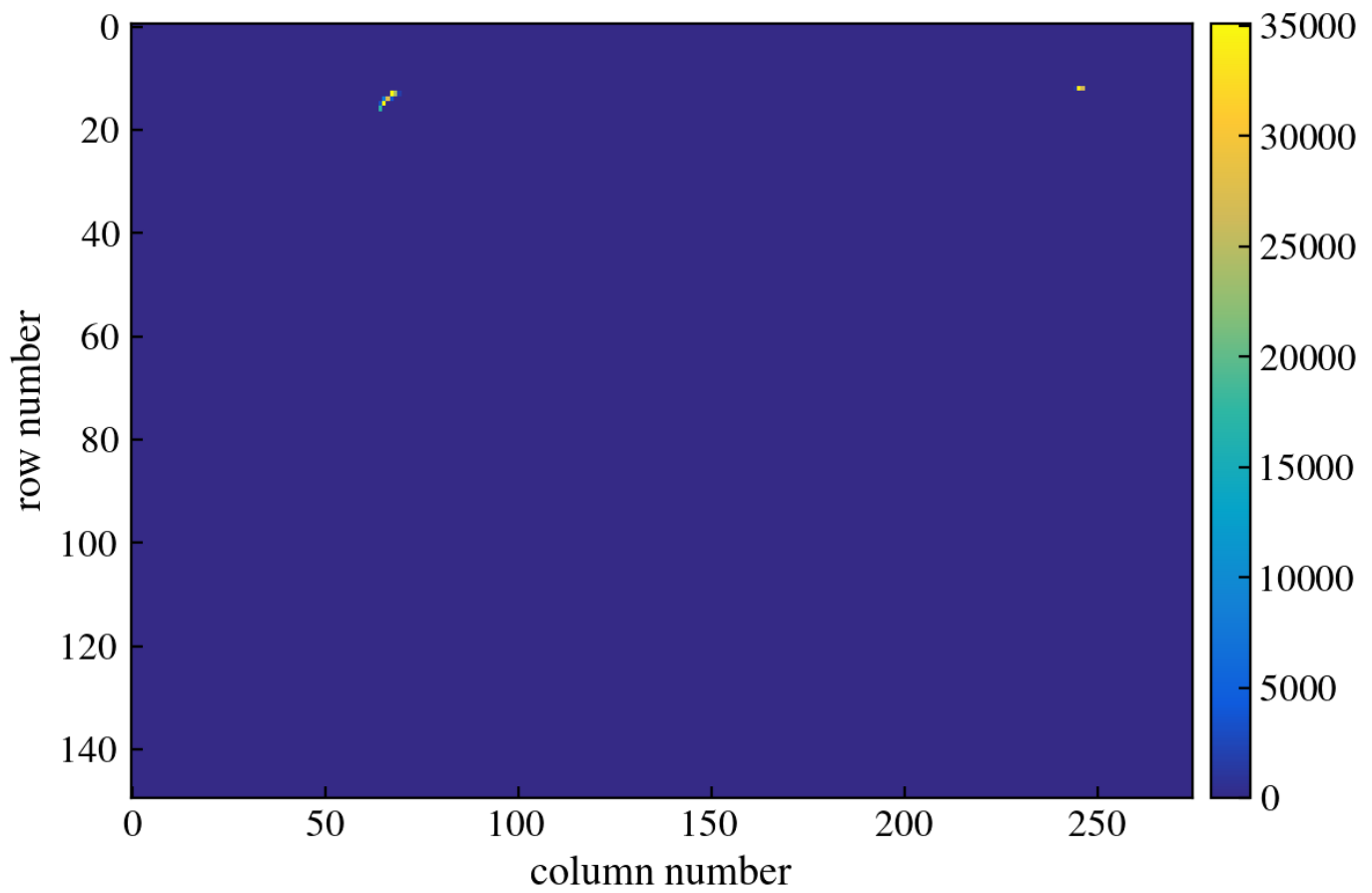
Figure 165: CCD Image
