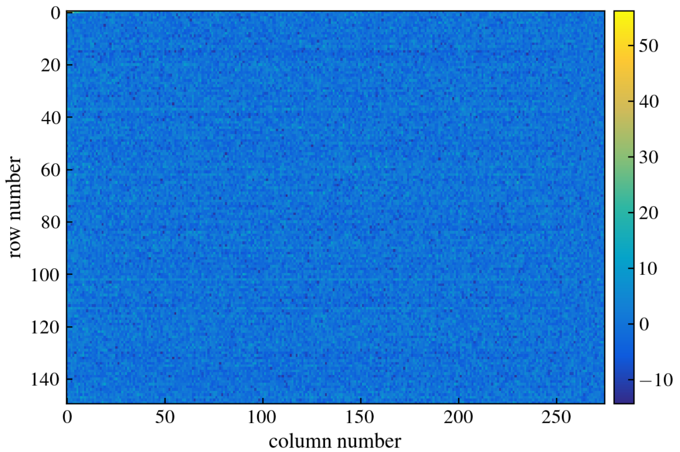
Figure 133: CCD Image
