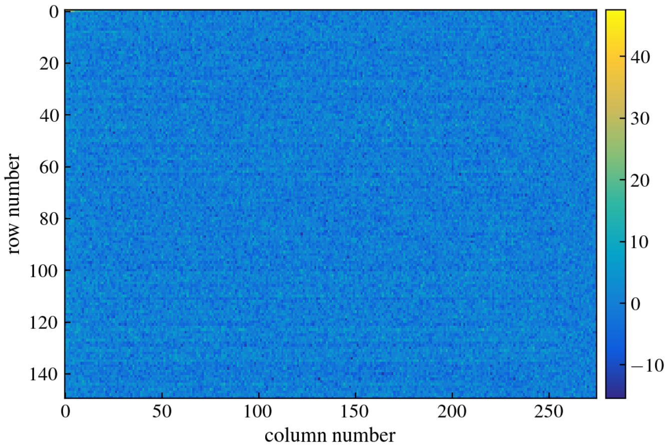
Figure 350: CCD Image
