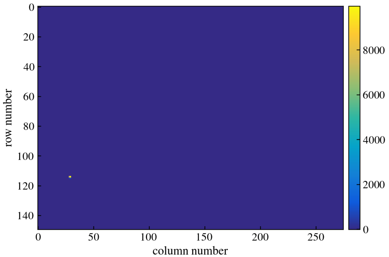
Figure 31: CCD Image
