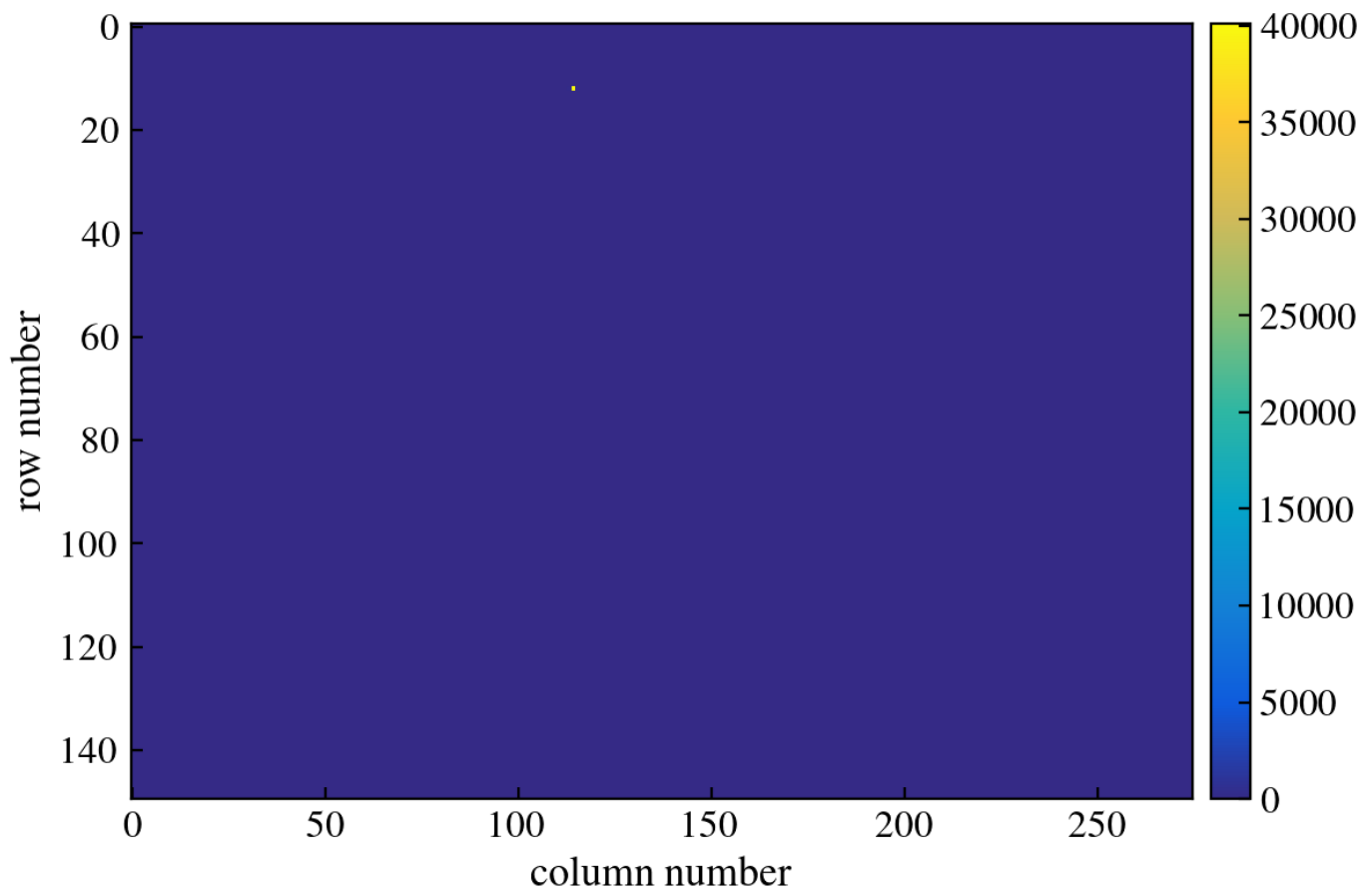
Figure 355: CCD Image
