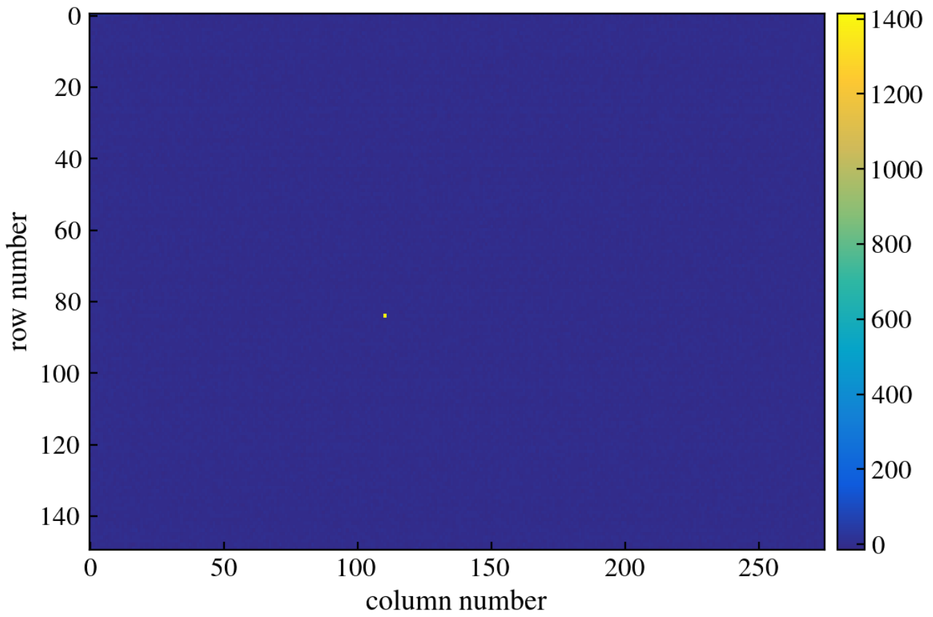
Figure 332: CCD Image
