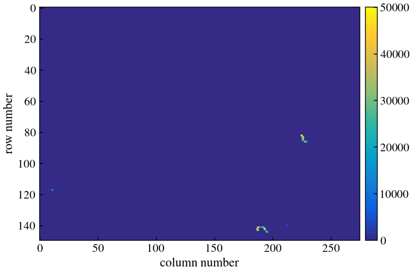
Figure 138: CCD Image
