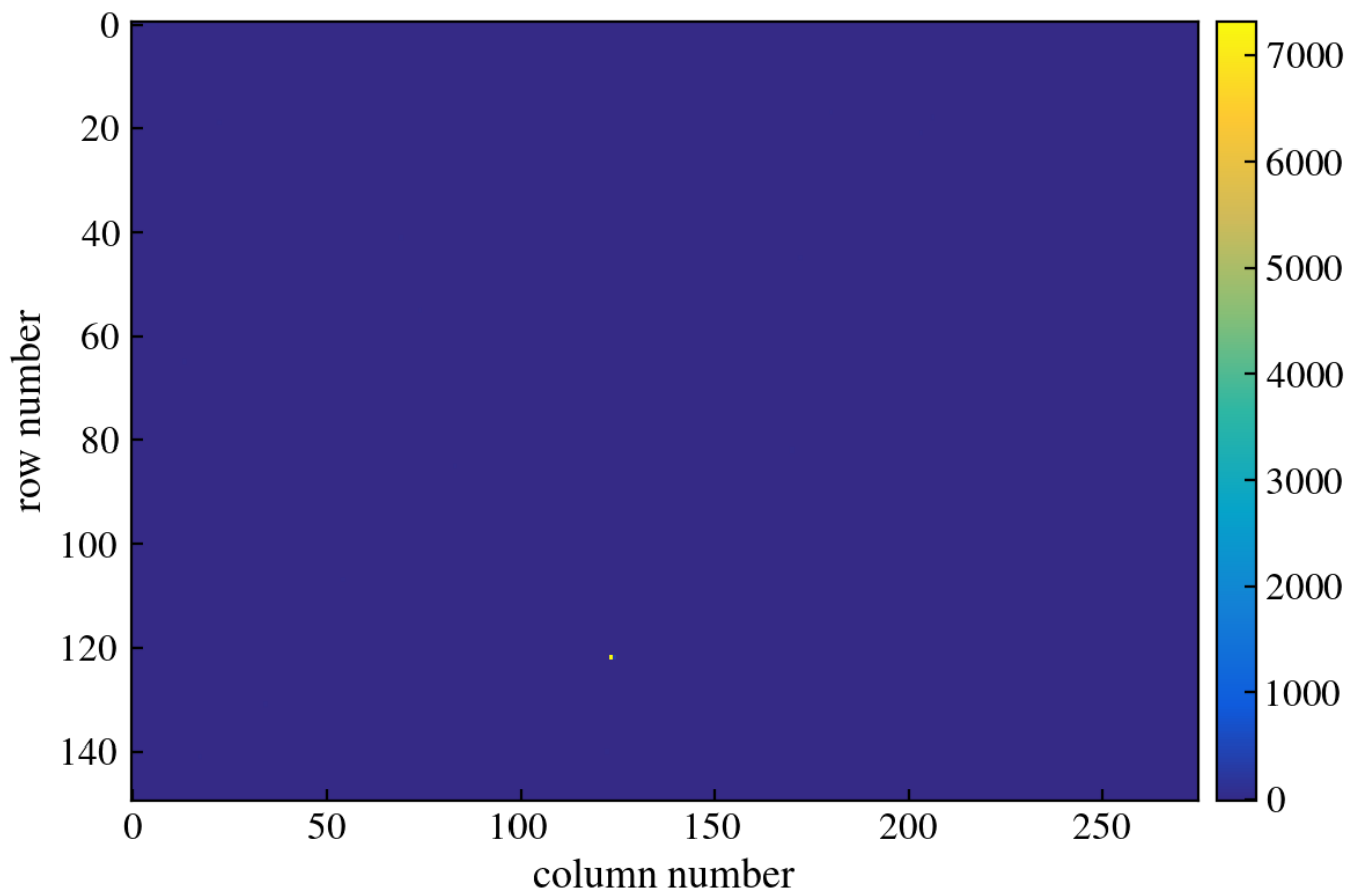
Figure 96: CCD Image
