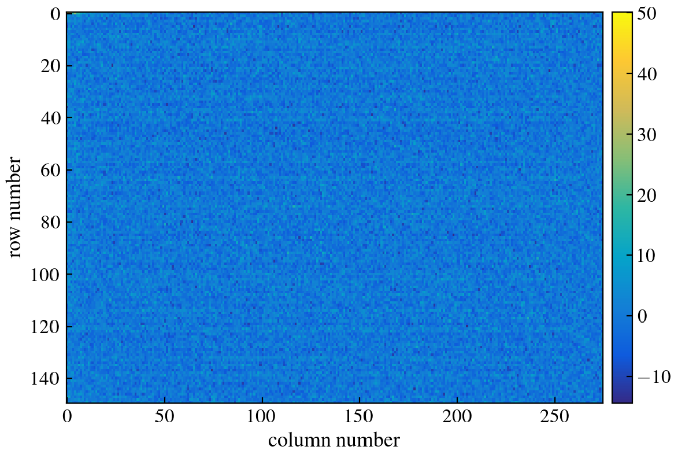
Figure 50: CCD Image
