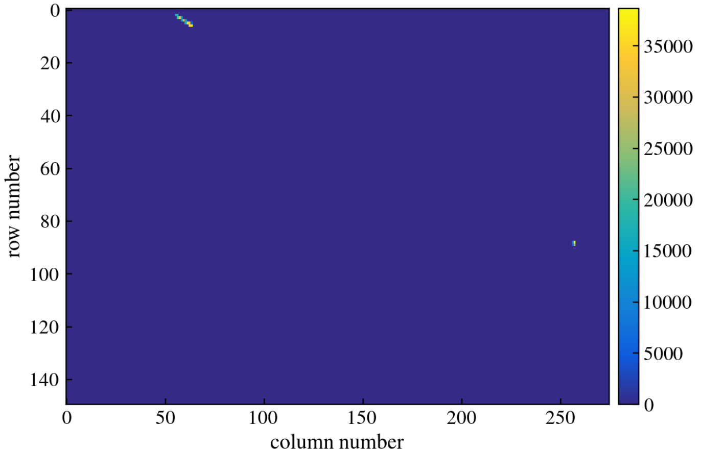
Figure 330: CCD Image
