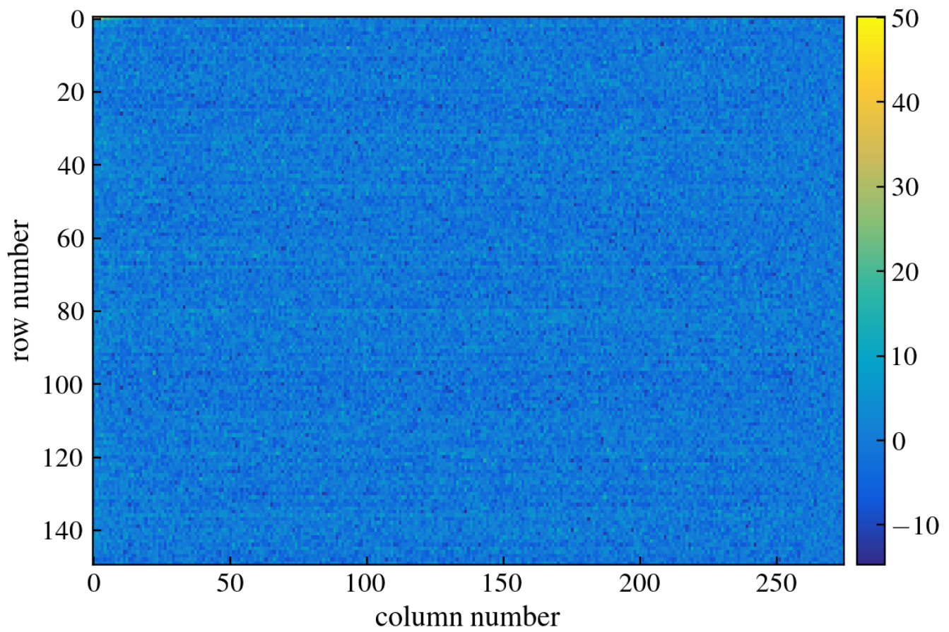
Figure 242: CCD Image
