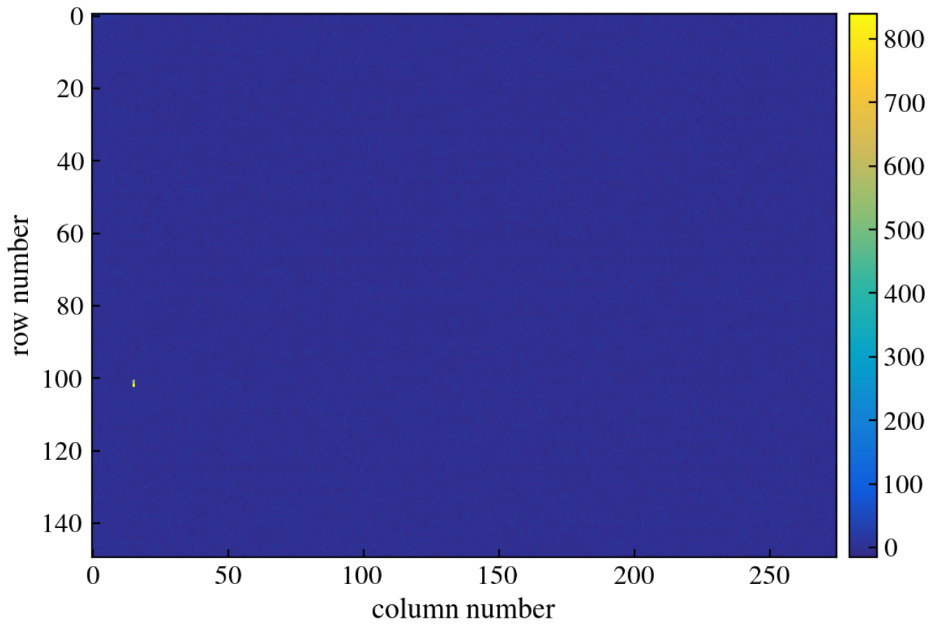
Figure 162: CCD Image
