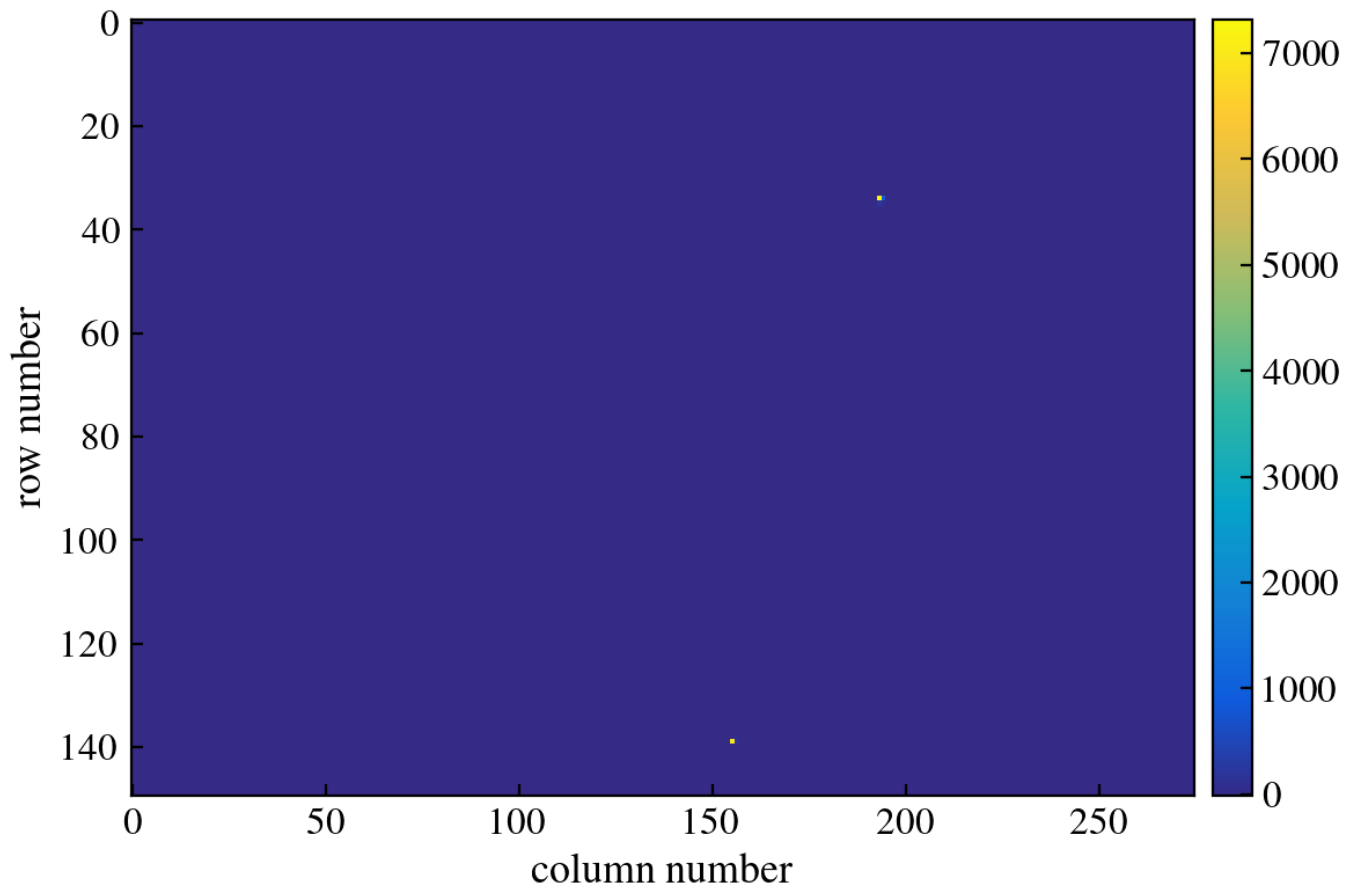
Figure 56: CCD Image
