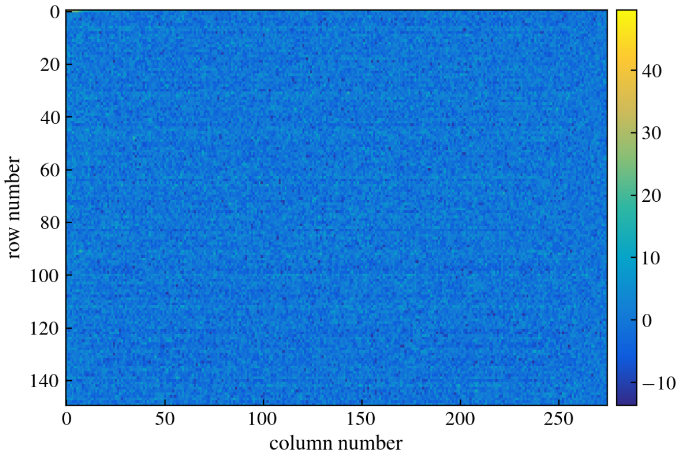
Figure 62: CCD Image
