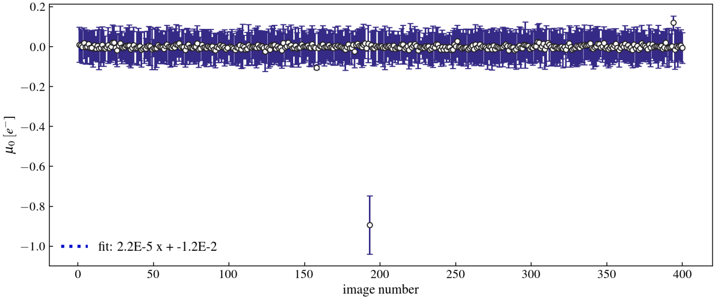
Figure 26: Overscan. PCD Gaussian fit: \mu_0
