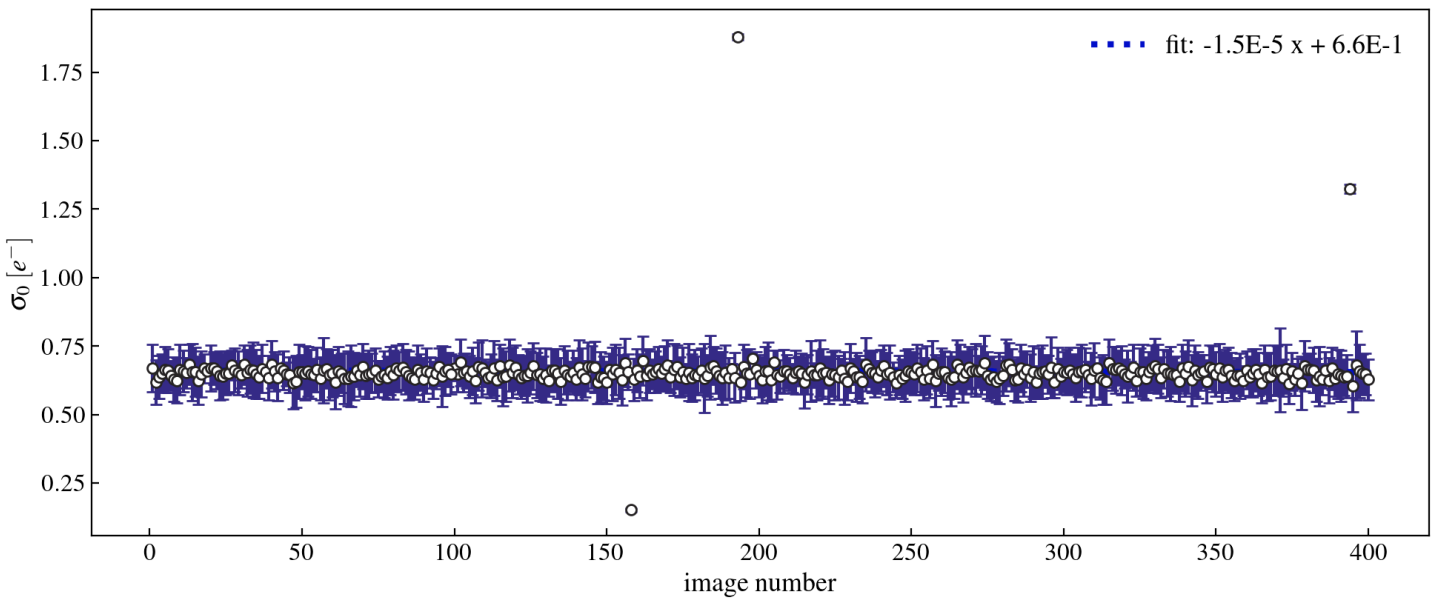
Figure 27: Overscan. PCD Gaussian fit: \sigma_0
