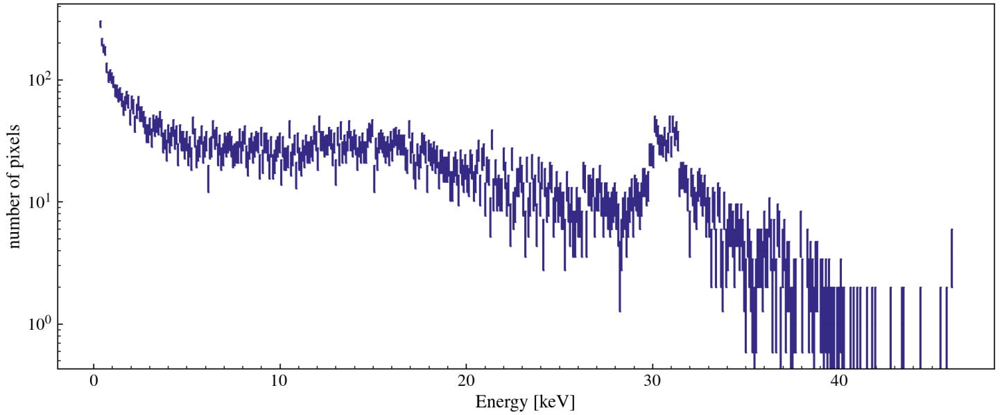
Single Pixel Energy Distribution [w/ 5.23 ADC/e- and 3.74eV/e-] [class MESinglePED]
