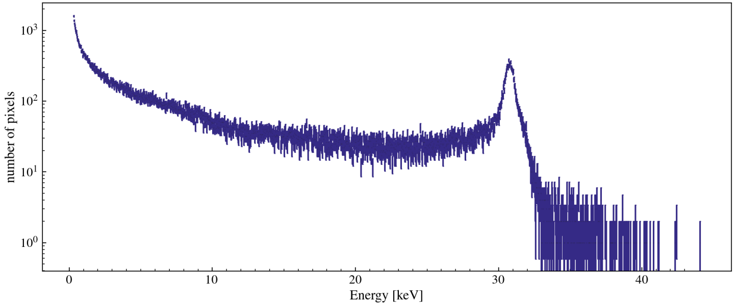
Single Pixel Energy Distribution [w/ 5.28 ADC/e- and 3.74eV/e-] [class MESinglePED]
