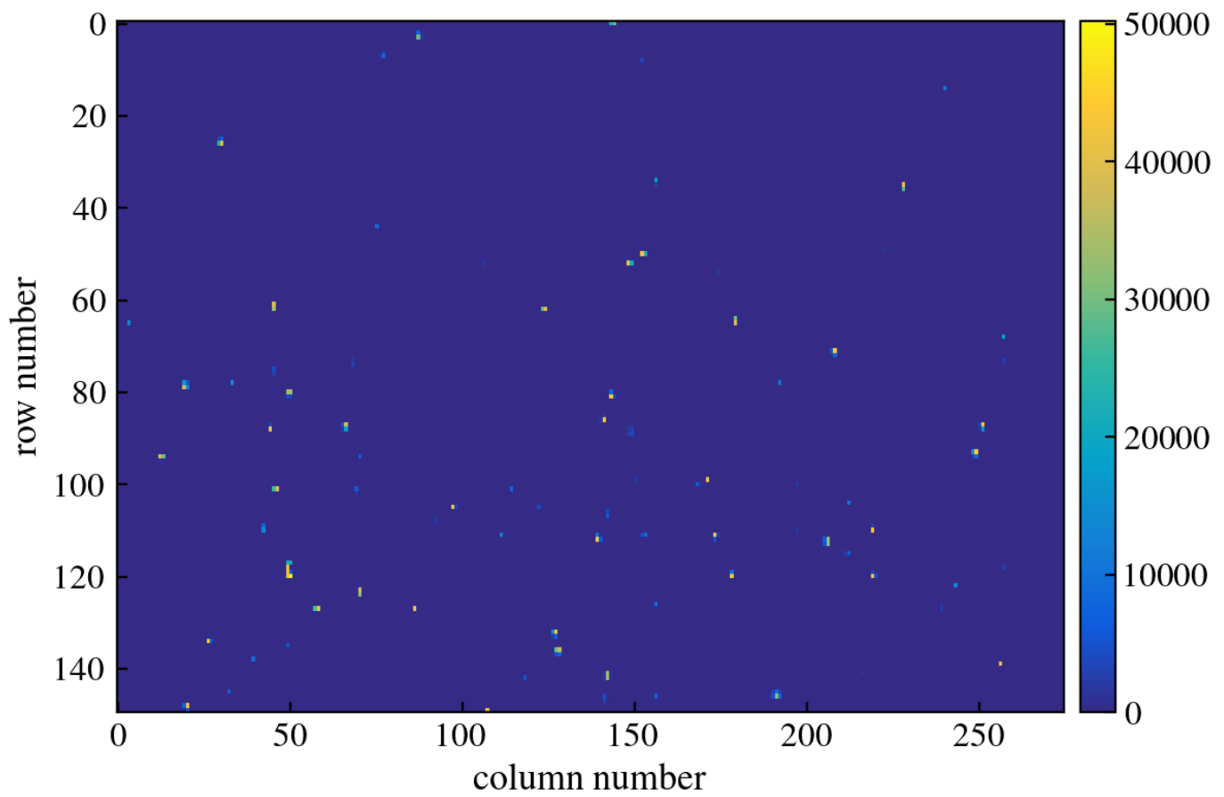
Figure 418: CCD Image
