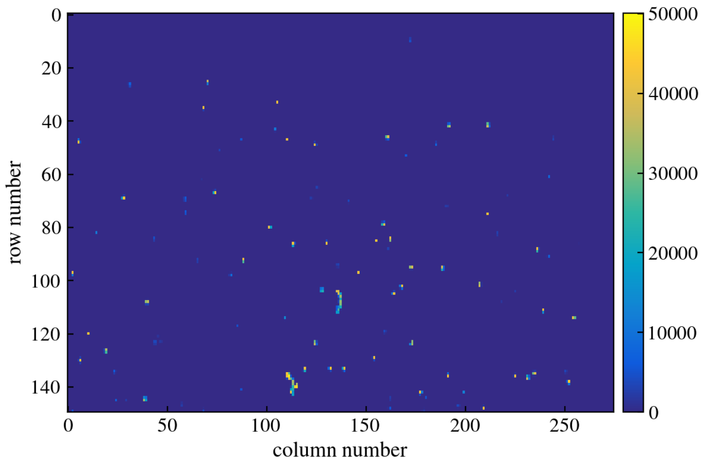
Figure 66: CCD Image
