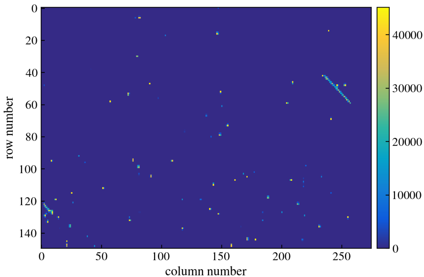
Figure 188: CCD Image
