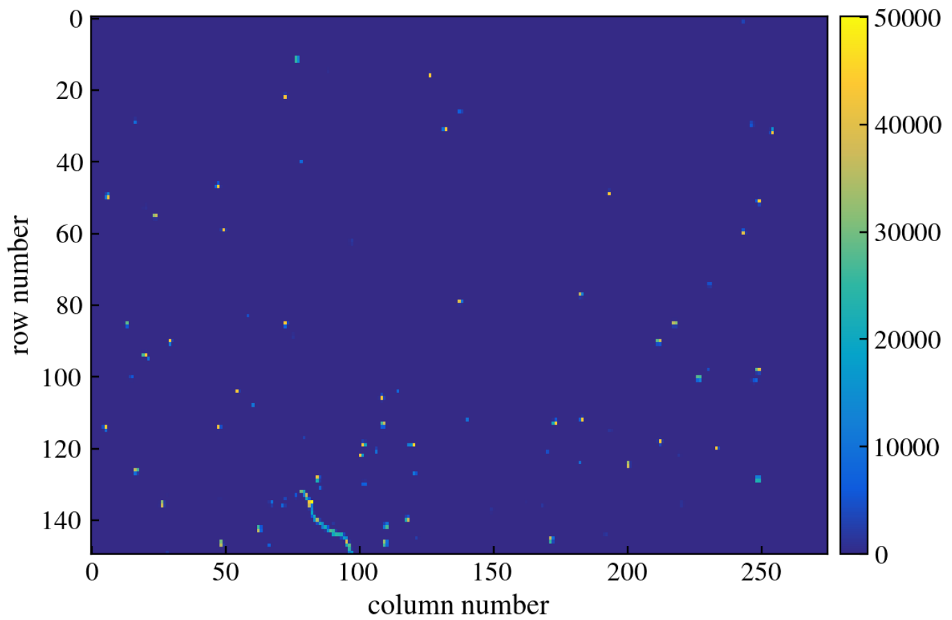
Figure 381: CCD Image
